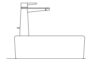
SINGLE-LEVER BASIN MIXER IN COMBINATION WITH A SURFACE-MOUNTED/BUILT-IN WASHBASIN WITH TAP LEDGE
