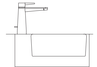
SINGLE-LEVER BASIN MIXER IN COMBINATION WITH AN UNDERCOUNTER/BUILT-IN WASHBASIN
